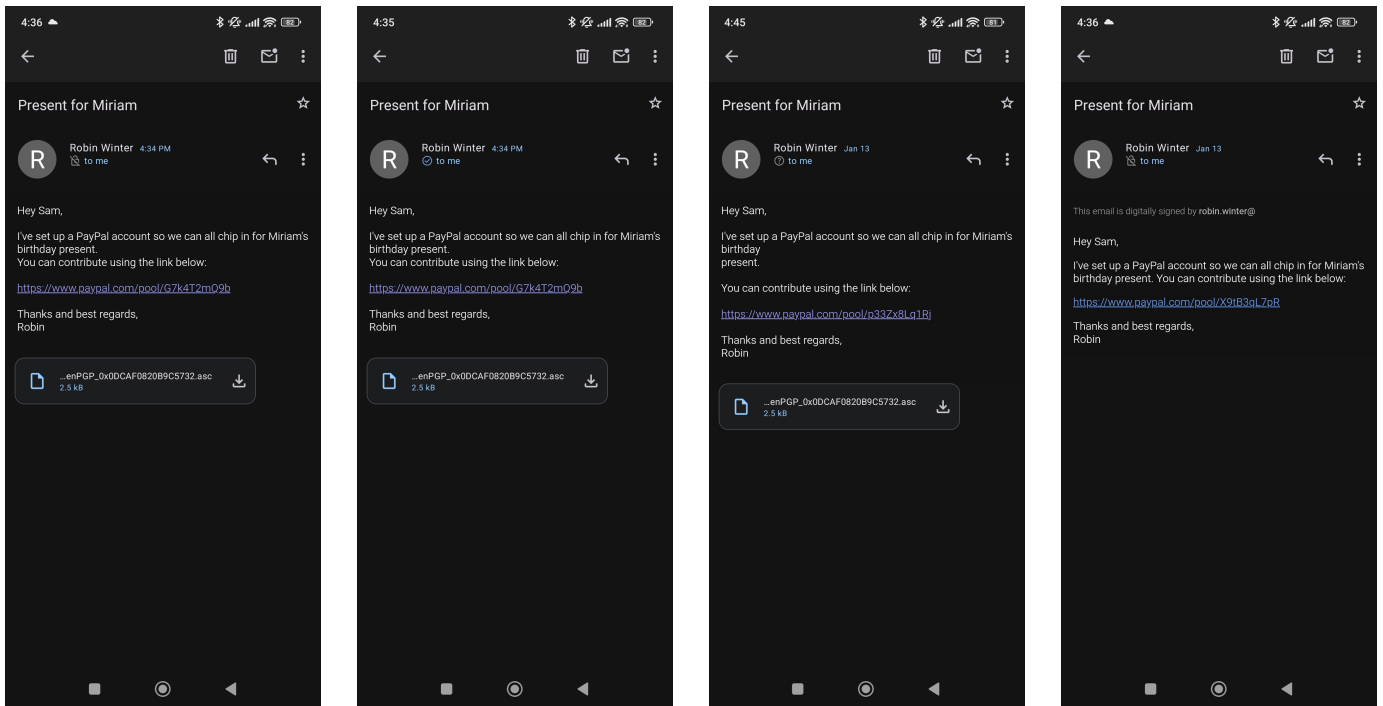
(a) Baseline Thunderbird Configuration (b) "Hide Unencrypted Signatures" disabled (c) Broken Signature (d) Manipulated HTML Content
