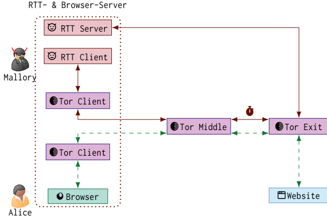
Figure 4: The experimental setup for our side-channel attack. The dashed green lines depict the victim’s communication. The straight red lines depict the adversary’s communication. The adversary is in control of the RTT client and server and measures the RTT between the middle and exit relay.
