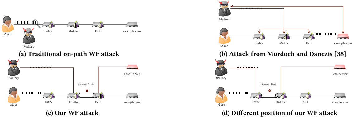
Figure 2: In a traditional WF attack (a), Mallory is in the position of Alice during the training phase and trains the ML model. During the prediction phase, Mallory needs to be on-path, analyze traffic, and predict which website Alice has visited. In the attack by Murdoch and Danezis [38] (b), the attacker controls a Tor relay and a website (corrupted server) and sends specific patterns over that server, which are detectable by the RTT measurements. In our WF attack (c), Mallory is off-path for both phases and builds a two-hop circuit with a specific middle and exit relay. During the training phase, Mallory collects RTT traces between two relays while performing website accesses from Alice’s position. Mallory uses these traces to train an ML model. To predict a website Alice visits, Mallory collects new RTT traces from Alice’s traffic and uses the ML model to predict the websites Alice visits. In (d), our website fingerprinting attack measures the RTT fluctuations between guard and middle relay instead of middle to exit relay.
