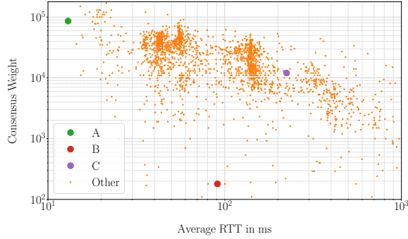
Figure 5: This shows the average RTT in ms against the weight in the consensus measure. The RTT is measured from our middle relay. Our chosen exit relays are marked.
