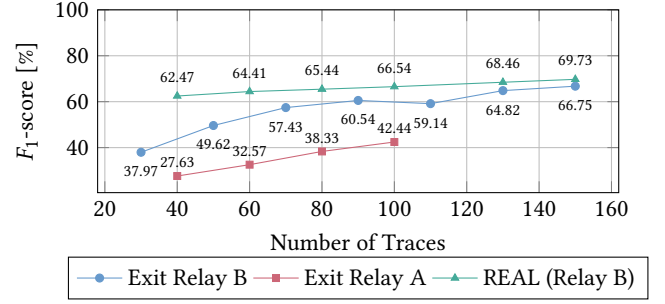
Figure 10: F_1 -score depended on the number of traces for exit relays A and B and for the REAL experiment on exit relay B. The results indicate that increasing the number of traces improves the classification performance.
