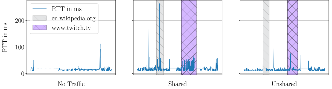
Figure 3: Sample RTT measurements for two websites under different scenarios. Shared means the middle and exit relays are the same for the attacker and the victim. Unshared means both have the same middle relay but a different exit relay.
