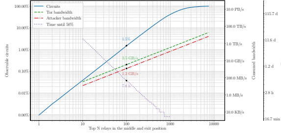
Figure 9: How many circuits an attacker could observe, the impact on the bandwidth, and the time duration. The x-axis refers to the top N most likely relays in the middle and exit position that an attacker could pick. All lines share the same x-axis but use a different y-axis. The blue line, which is the observable circuits in percent, uses the y-axis on the left side. The green and red lines, Tor and attacker bandwidth, use the first y-axis to the right. The lila line, time duration until 50 %, uses the second y-axis to the right.
