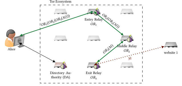
Figure 1: Example of how Tor works. Alice’s Tor client first contacts the Directory Authority (DA) to get a list of Onion Routers (ORs). Then it encrypts her message M three times in reverse order and sends it to the first Tor relay, also referred to as the Tor entry relay. The straight green line contains traffic that Tor encrypts, and the dotted red line is traffic that might or might not be encrypted.
