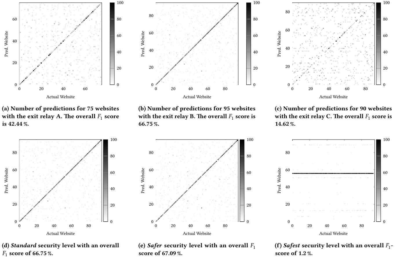
Figure 6: Subfigure (a)–(c) shows the number of predictions for each website measured from our middle relay to exit relay A, B, and C. Subfigure (d)–(f) shows the number of predictions for 95 websites with different security levels measured from our middle relay to exit relay B. For all subfigures, the actual website is shown on the x axis, the website predicted by the model is shown on the y axis.
